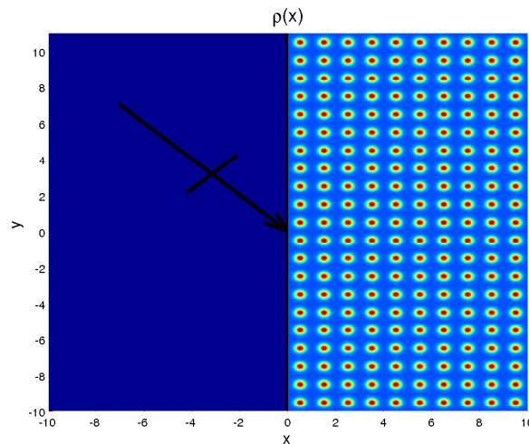
Figure 1. The refraction index in the two half space and the direction of the incident plane wave ( \theta = \pi/4 )
